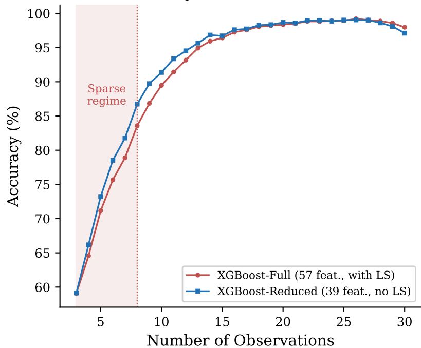
(a) Accuracy vs. Observation Count
