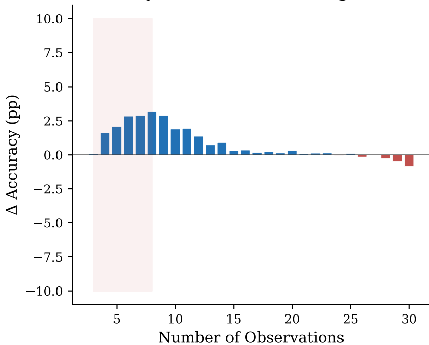
(b) Accuracy Gain from Removing LS Features
